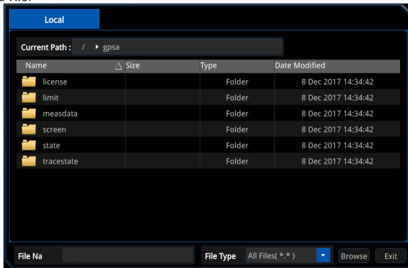
Figure 3-11 File Manager
