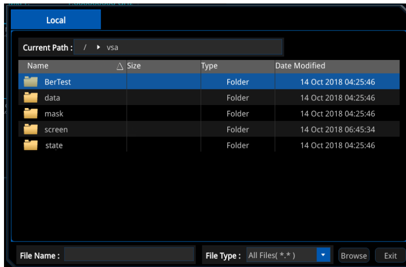
Figure 5-10 File Manager
