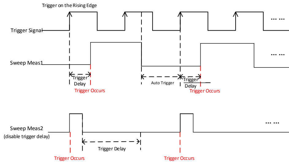
Figure 5-2 Relationship of Trigger Parameters
