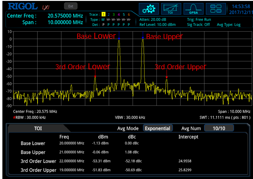
Figure 2-12 TOI Measurement Interface
