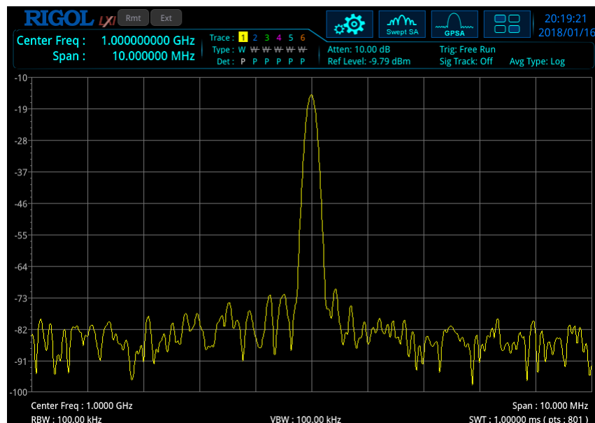
Figure 2-19 After Auto Search
