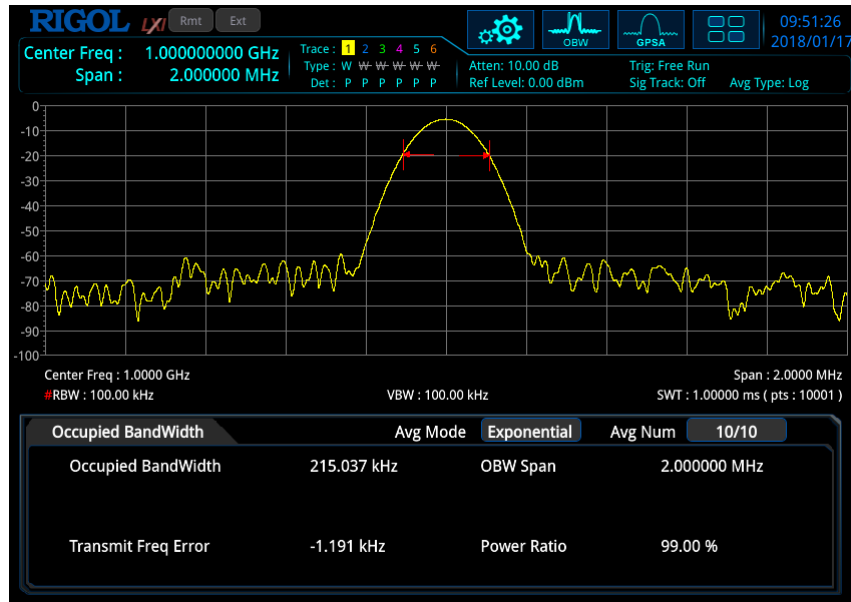
Figure 2-8 OBW Measurement Interface
