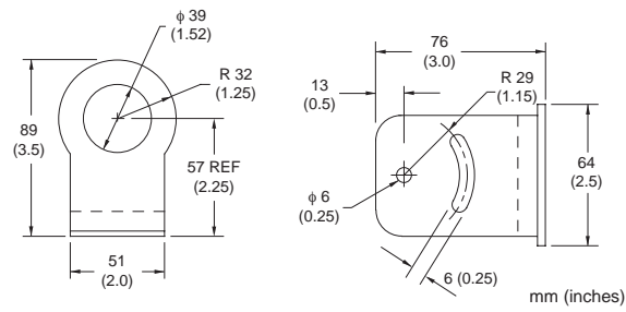
Figure B-5: Fixed Mounting Bracket
