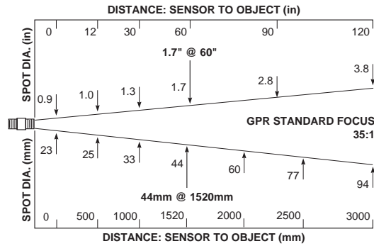
Figure B-12: GPR Standard Focus Optical Chart
