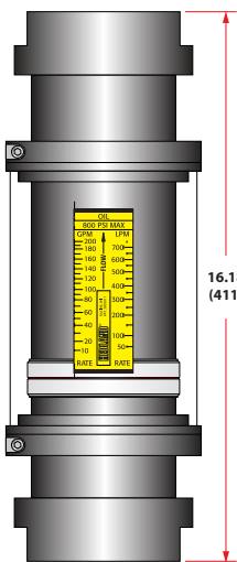
Figure 10: 3 inch; SAE, NPTF, BSPP Inches (mm)
