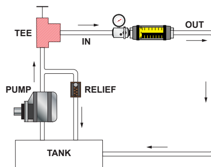
Figure 6: Pump test
