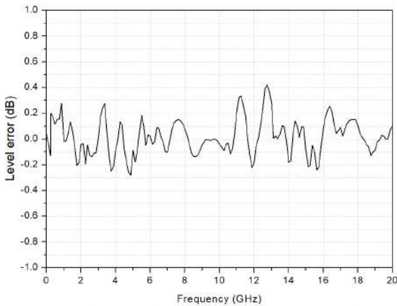
Measured at +10dBm, level error vs frequency
