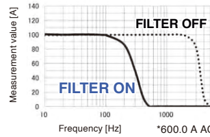
Frequency characteristics when using the filter*
