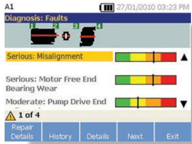
810 Vibration Tester
